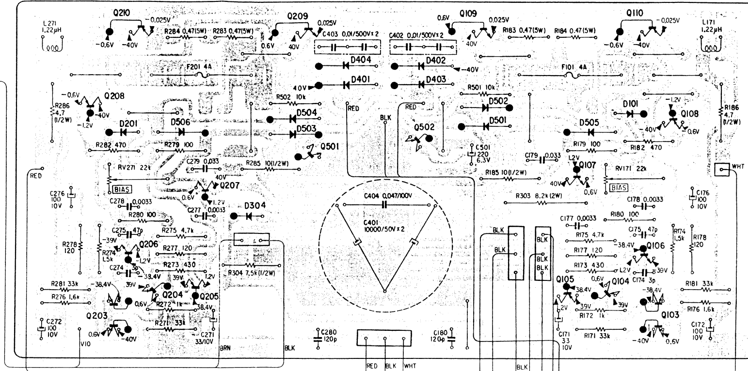
(POWER AMP BOARD)
